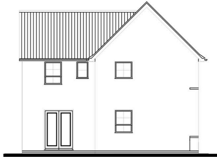
REAR ELEVATION Alderney
