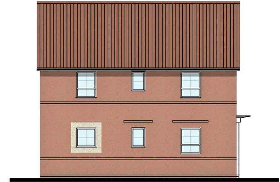
FRONT ELEVATION Alderney
