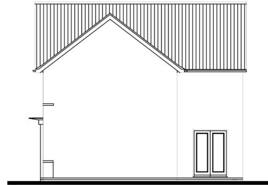
SIDE ELEVATION Alderney
